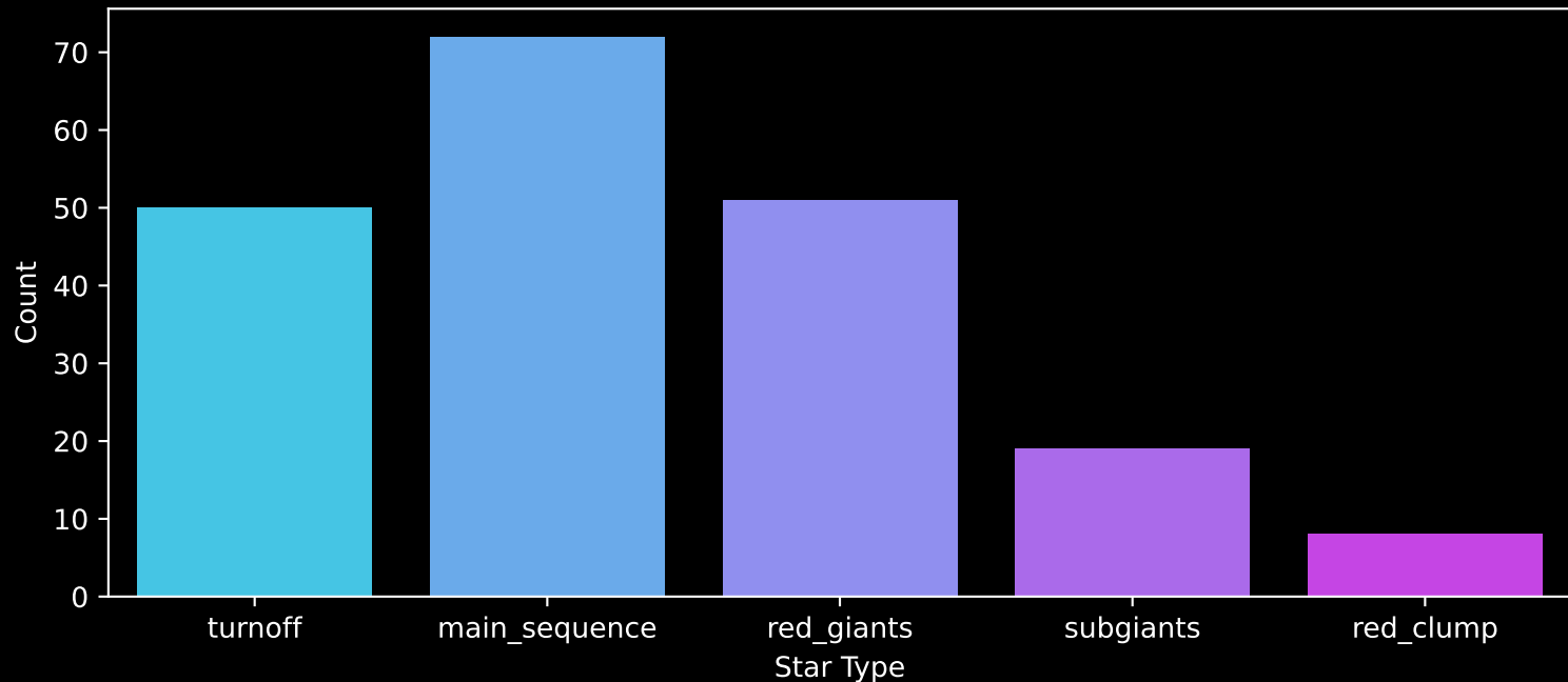
APOGEE DR17 Field: [K2_C7_014-15_btx] Count plot of Star Type
