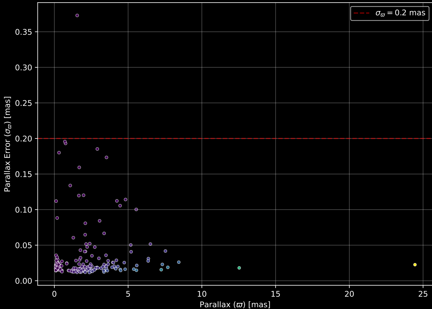
APOGEE DR17 Field: [K2_C7_014-15_btx] Parallax Quality (n= 200)
