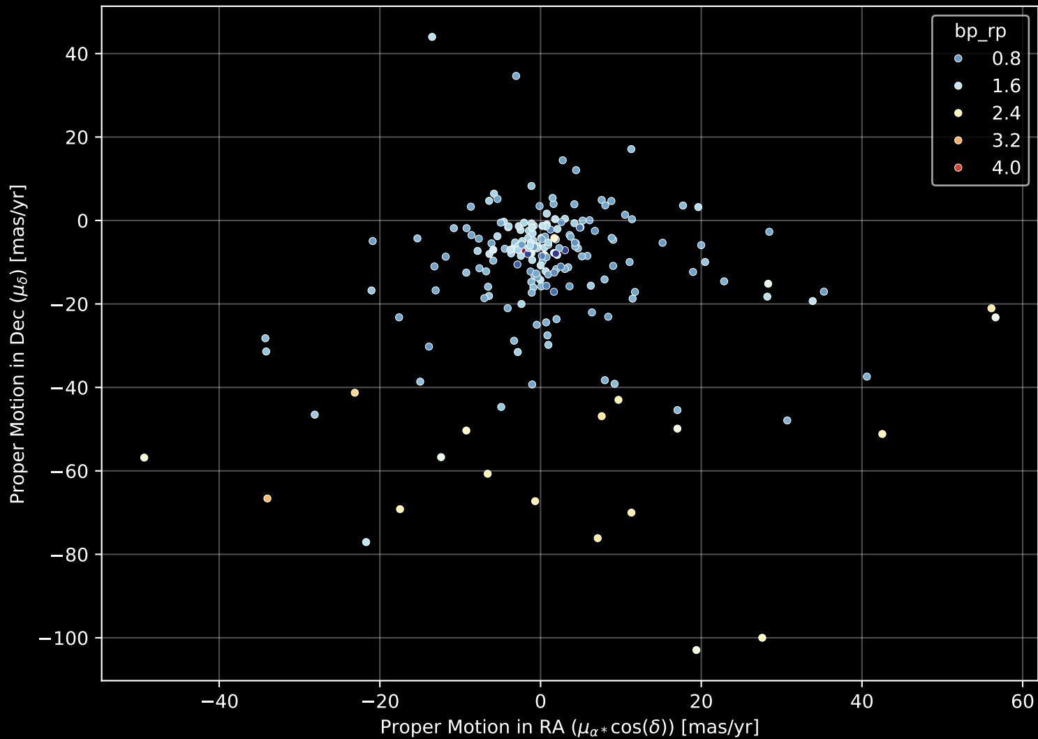
APOGEE DR17 Field: [K2_C7_014-15_bt] Proper Motion Diagram (n= 200)
