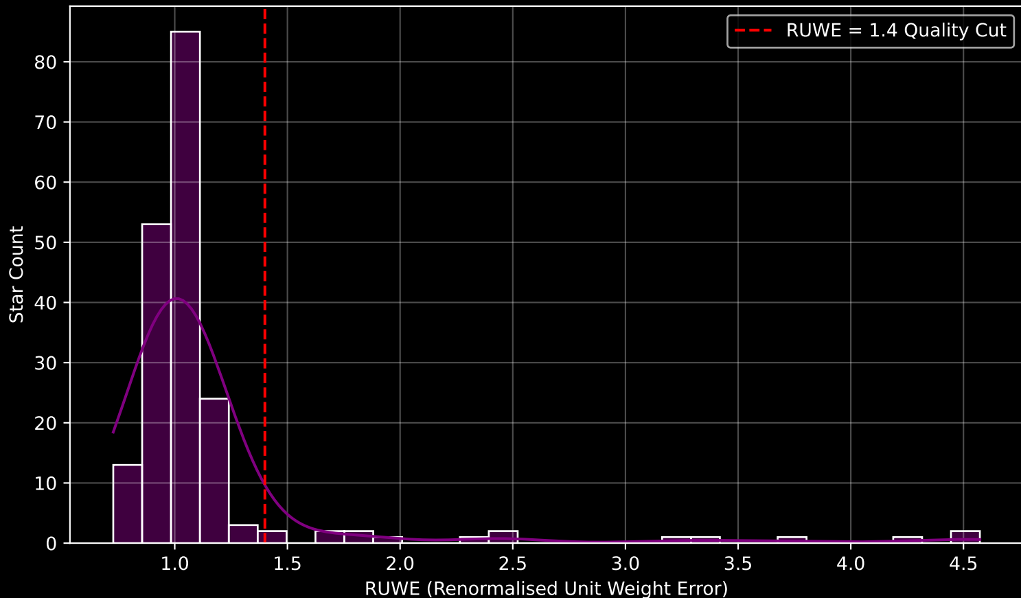
GAPOGEE DR17 Field [K2_C7_014-15_btx] RUWE Distribution (n= 194)
