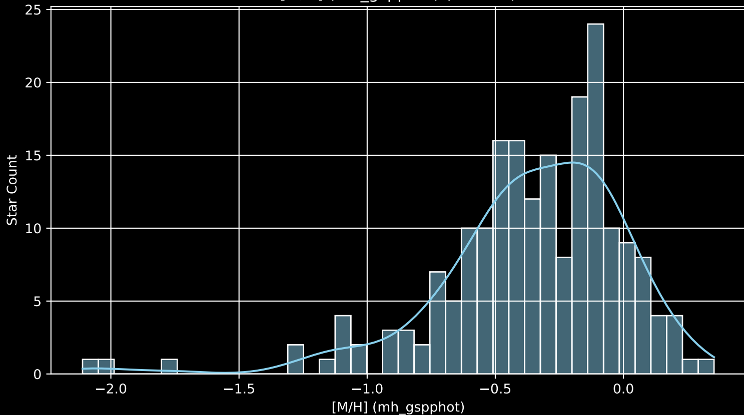
APOGEE DR17 Field: [K2_C7_014-15_btx [M/H] (mh_gspphot) (n= 199)
