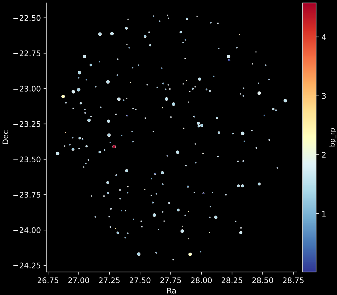
APOGEE DR17 Field: [K2_C7_014-15_btx] Stars: 200
